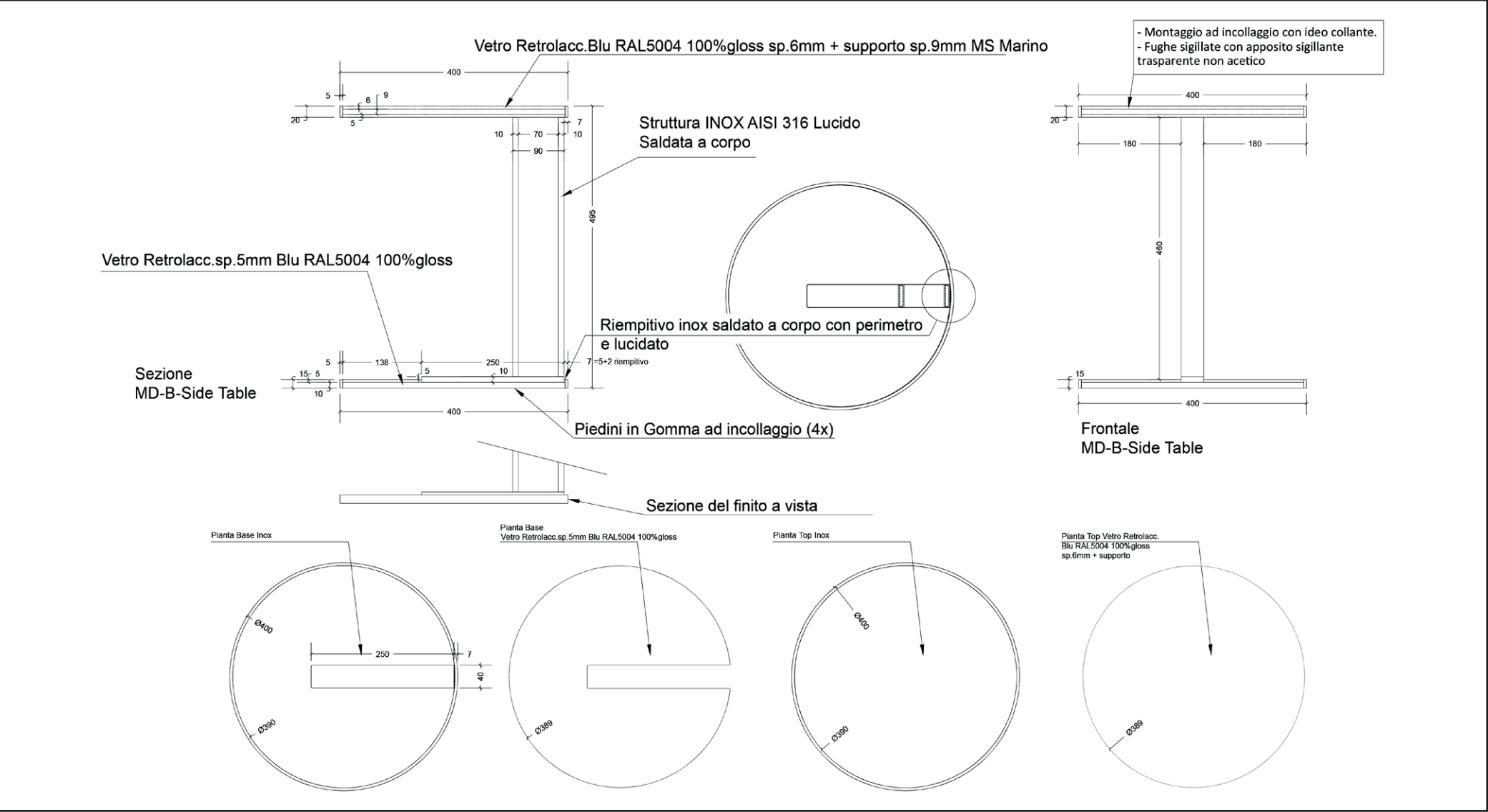
Side table - technical drawing
