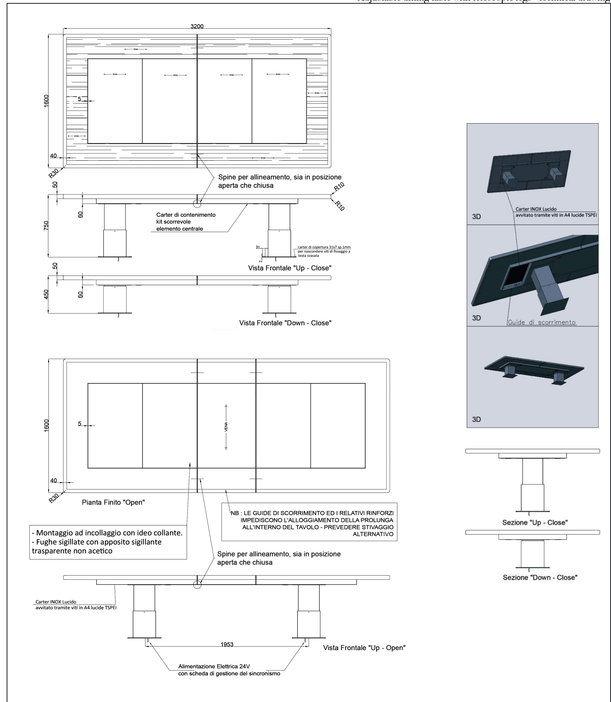
Adjustable dining table with telescopic legs - technical drawing
