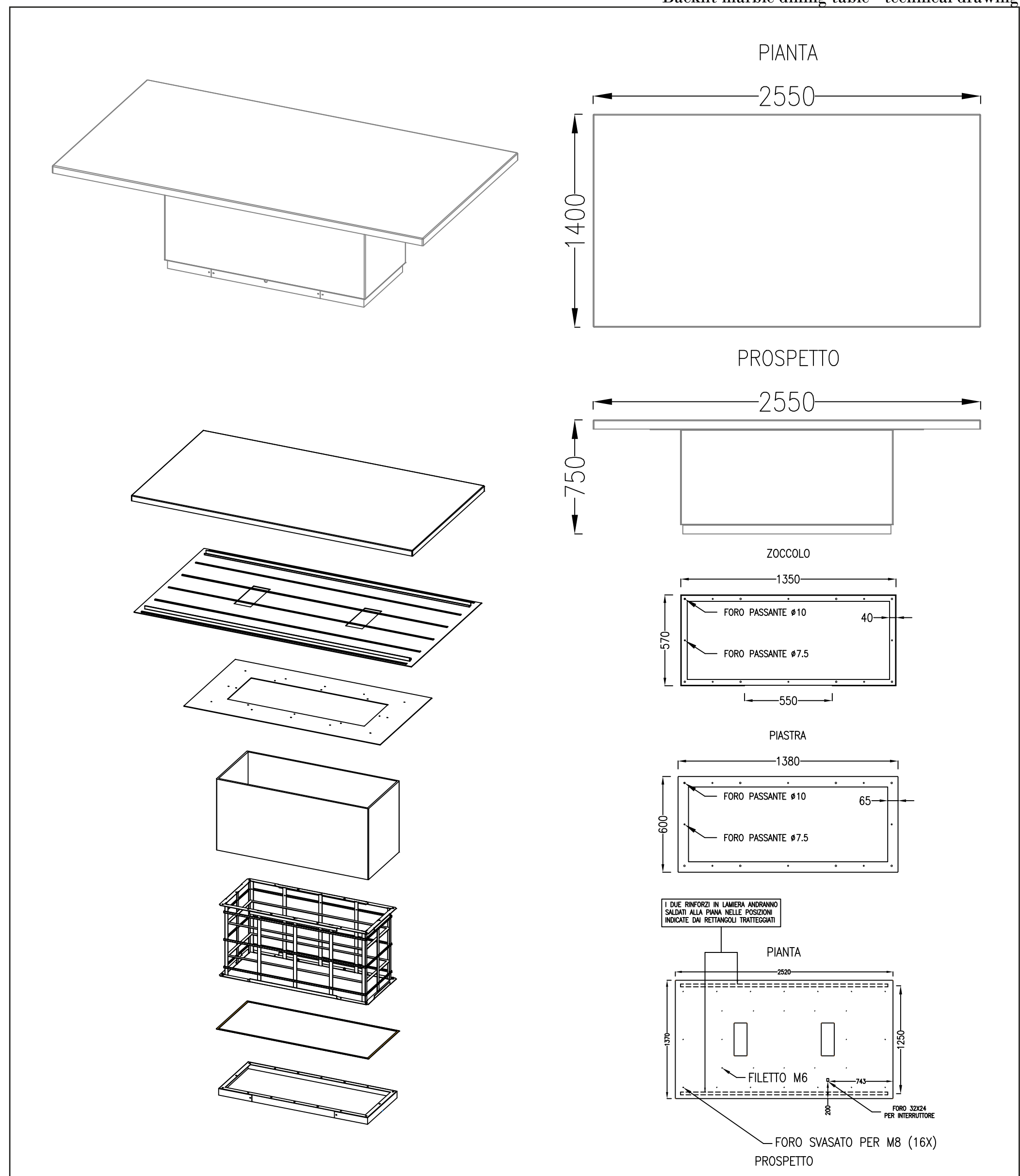
Backlit marble dining table - technical drawing
